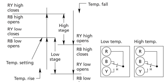
Figure 8 – Operational Sequence of Two-stage SPDT/SPDT Thermostats
