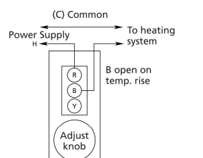
Figure 1 – Connection for a Typical Heating Control Circuit
