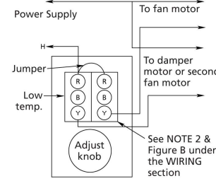
Figure 5 – Two-stage SPDT/SPDT Thermostats in Control of a Single-speed Ventilating Fan and Volume Increase Damper Motor
